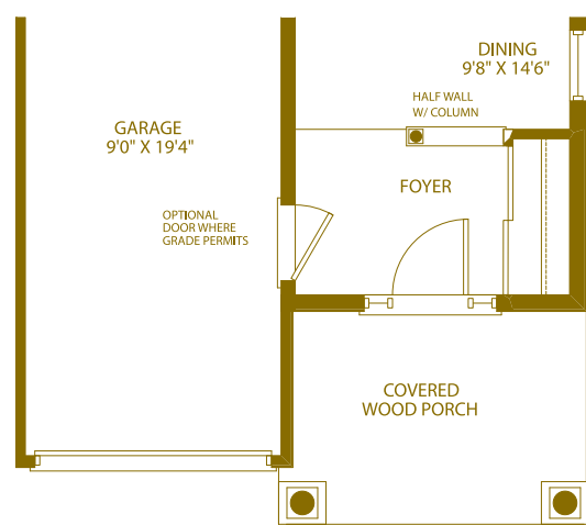
PARTIAL END PLAN GROUND FLOOR ARTS & CRAFTS
