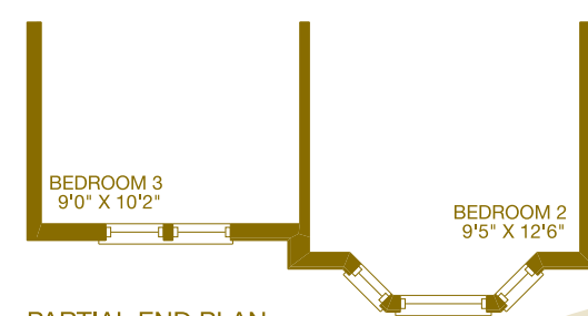
PARTIAL END PLAN SECOND FLOOR CANADIANA
