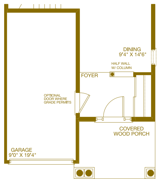
PARTIAL GROUND FLOOR ARTS & CRAFTS
