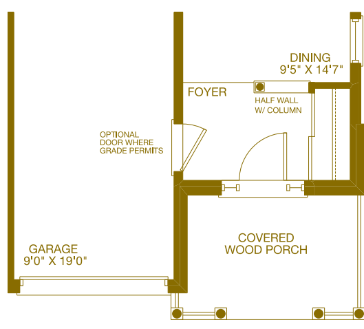
PARTIAL END PLAN GROUND FLOOR CANADIANA
