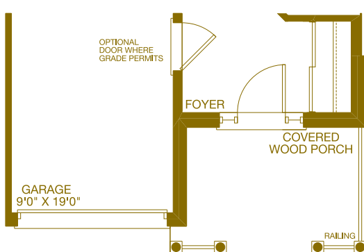
PARTIAL END PLAN GROUND FLOOR CANADIANA
