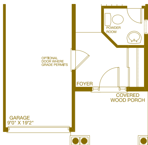
PARTIAL GROUND FLOOR ARTS & CRAFTS
