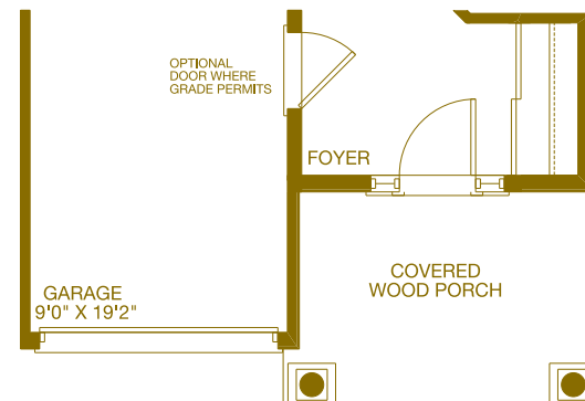
PARTIAL END PLAN GROUND FLOOR ARTS & CRAFTS
