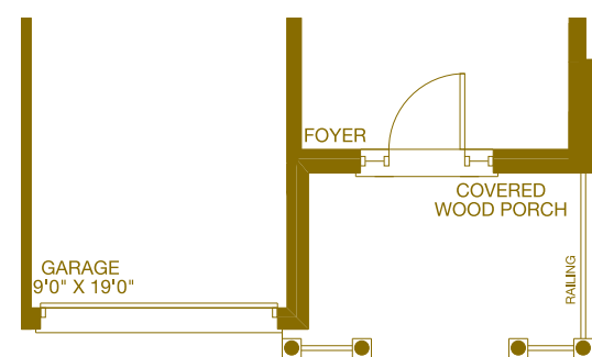
PARTIAL END PLAN GROUND FLOOR CANADIANA
