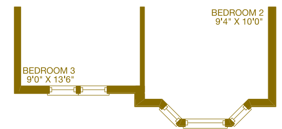
PARTIAL END PLAN SECOND FLOOR CANADIANA
