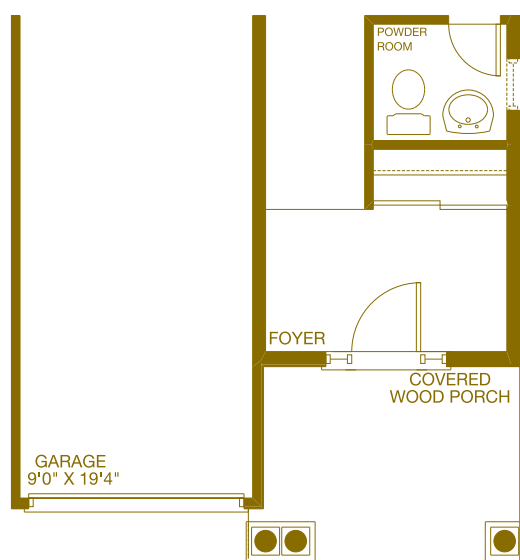
PARTIAL GROUND FLOOR ARTS & CRAFTS
