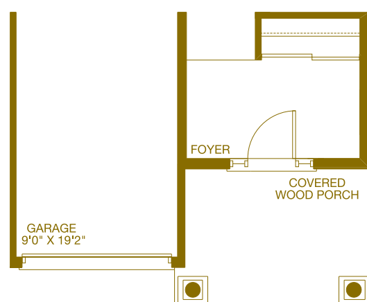
PARTIAL END PLAN GROUND FLOOR ARTS & CRAFTS
