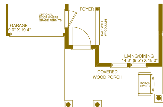
PARTIAL GROUND FLOOR - ARTS & CRAFTS
