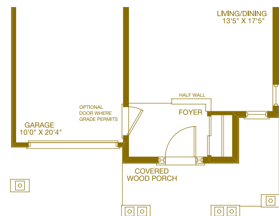
PARTIAL GROUND FLOOR ARTS & CRAFTS
