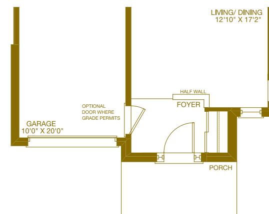
PARTIAL GROUND FLOOR GEORGIAN
