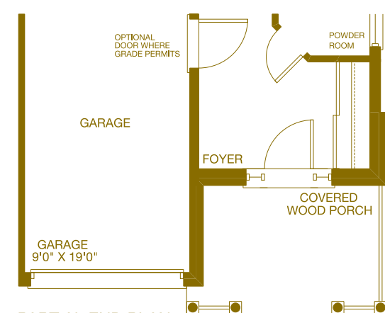
PARTIAL END PLAN GROUND FLOOR CANADIANA
