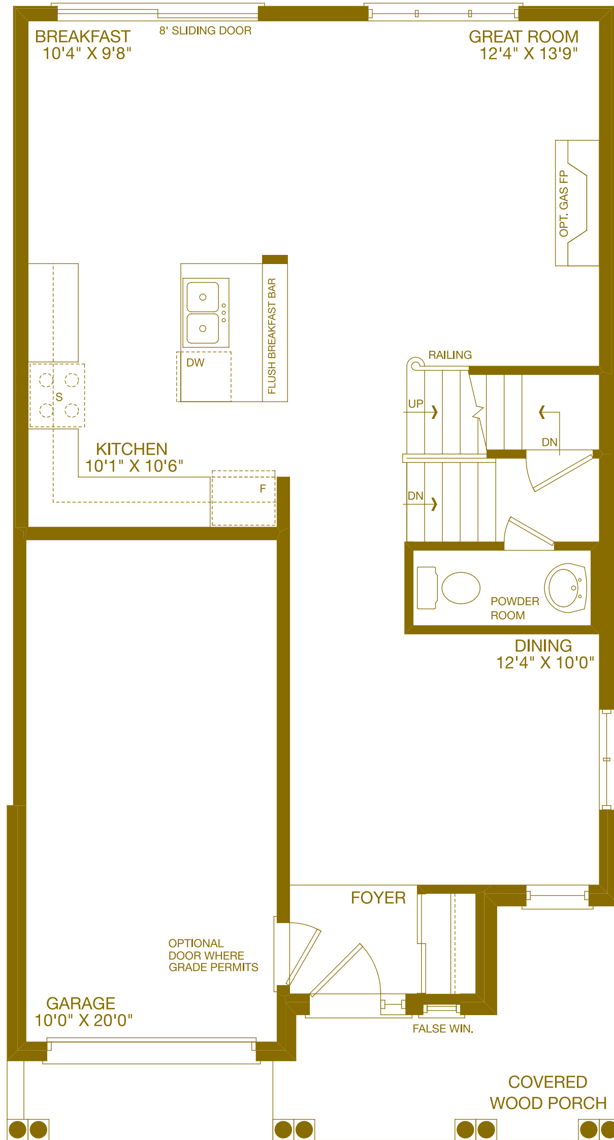
GROUND FLOOR CANADIANA
