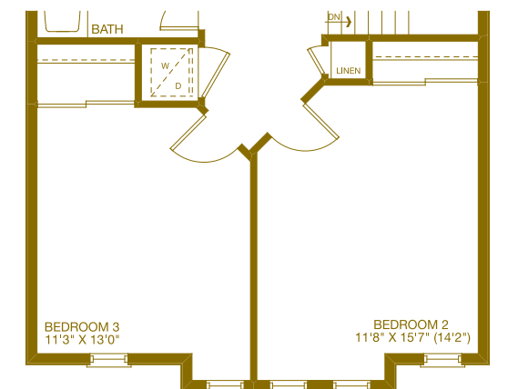
PARTIAL SECOND FLOOR GEORGIAN
