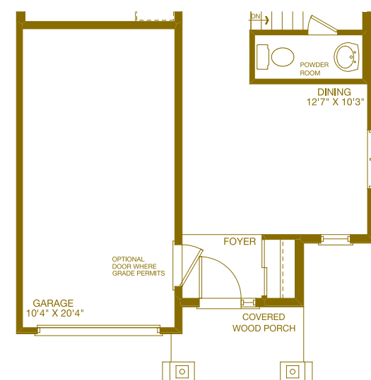
PARTIAL GROUND FLOOR ARTS & CRAFTS
