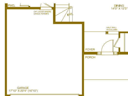
PARTIAL GROUND FLOOR GEORGIAN
