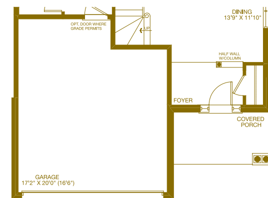
PARTIAL GROUND EDWARDIAN
