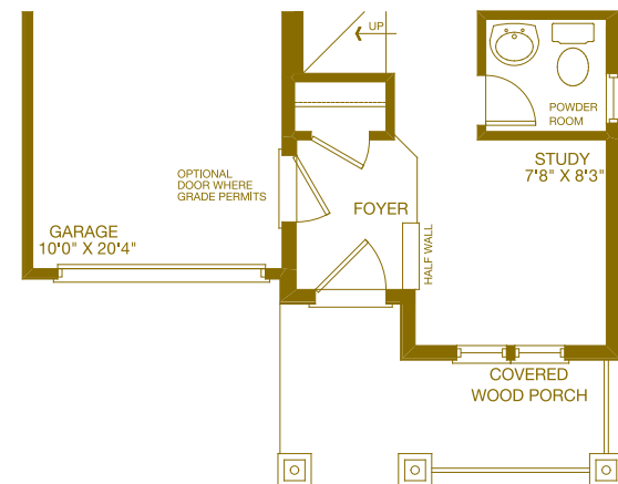
PARTIAL GROUND ARTS & CRAFTS
