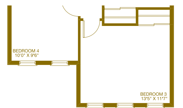
PARTIAL SECOND FLOOR GEORGIAN
